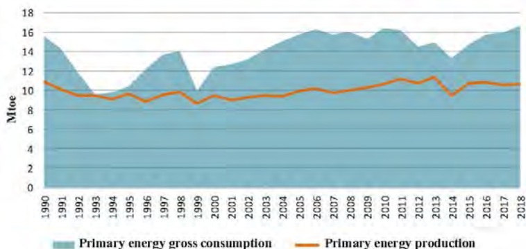
Figure 2. Primary energy consumption and production in the Republic of Serbia
