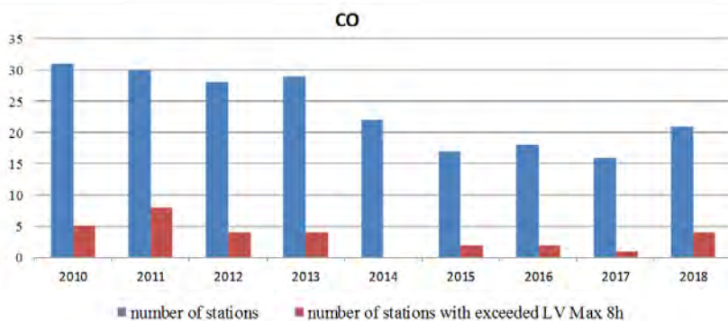
Figure 37. Comparative view of number of stations where carbon-monoxide is measures and number of stations where daily eight-hour limit value is exceeded
