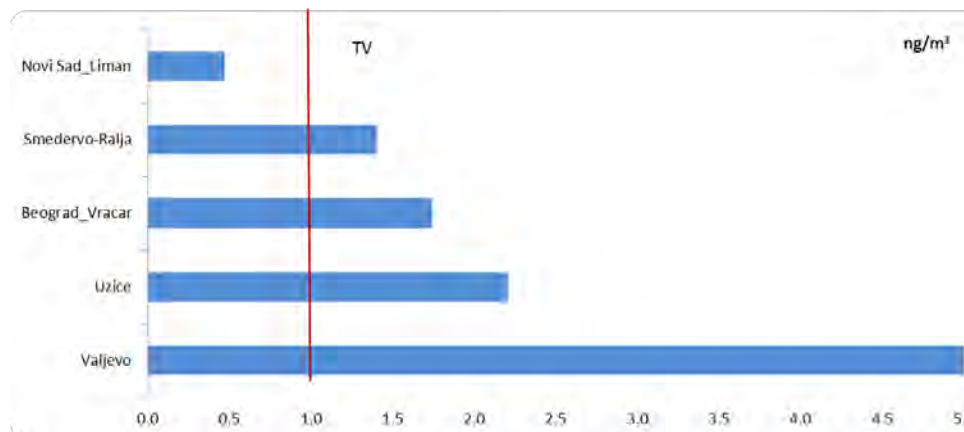
Figure 44. Mean annual value of benzo(a)pyrene in 2018
