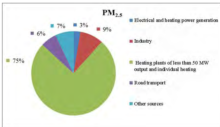
Figure 16. National emission balance for PM 2.5 per sector
