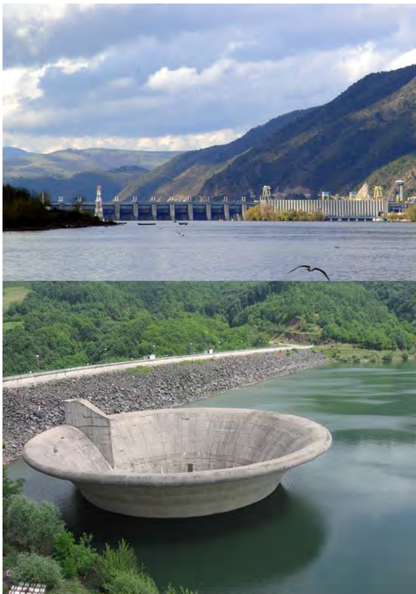
HPP Djerdap "EPS", The Barje Reservoir - the dam and bell-mouth spillway (Photo: D.Jovanovic)
